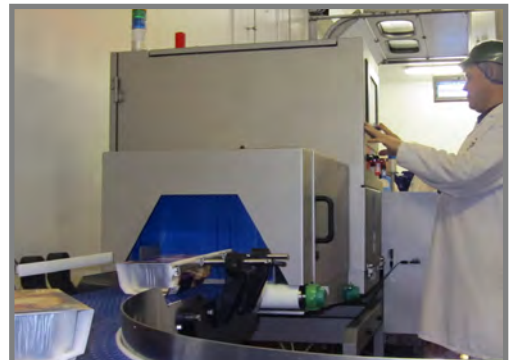
X-ray system inspects foil tray packed meat joints
